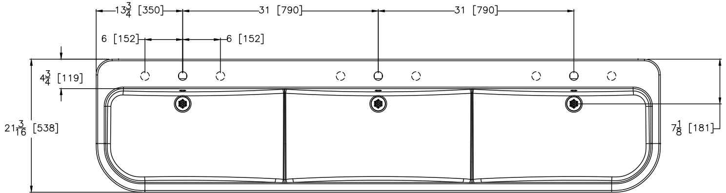
TOP VIEW
