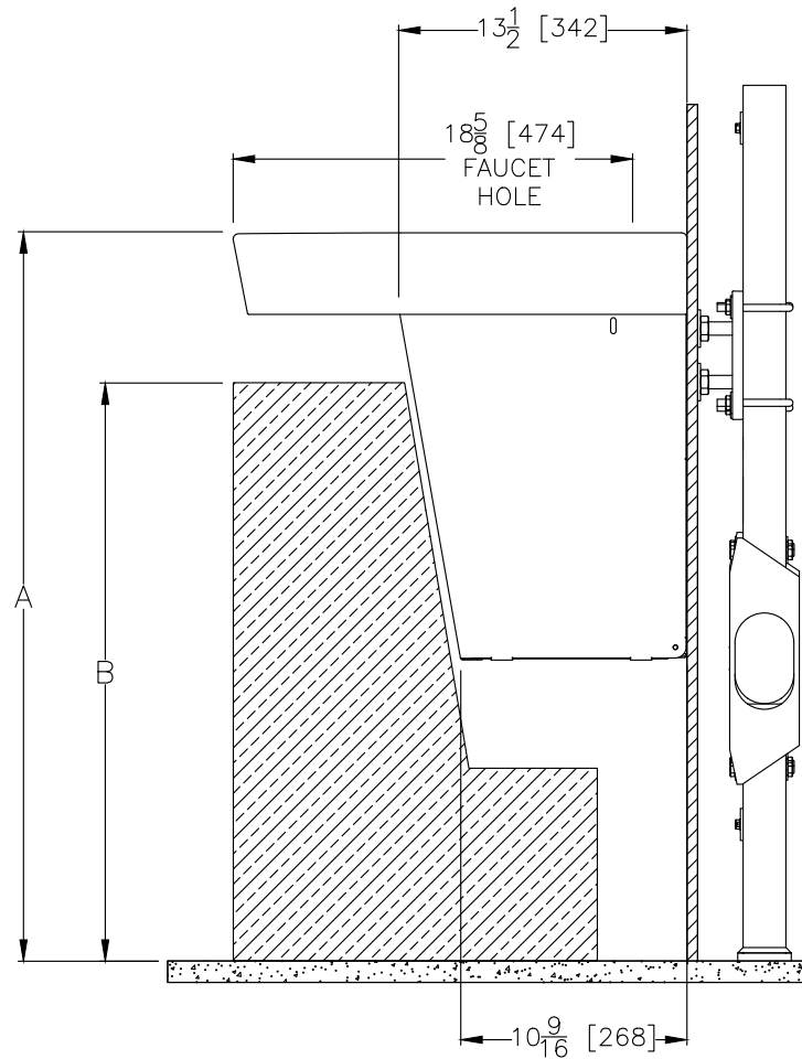
SIDE VIEW
