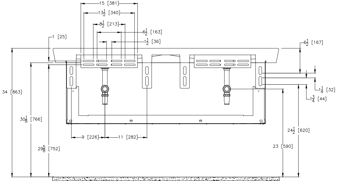
BRACKET VIEW
