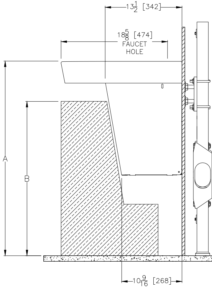
SIDE VIEW
