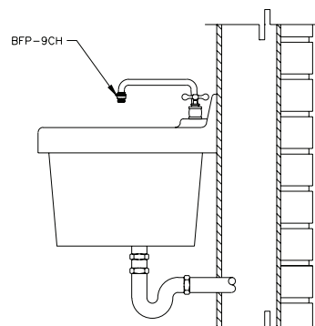
TYPICAL SERVICE SINK INSTALLATION
