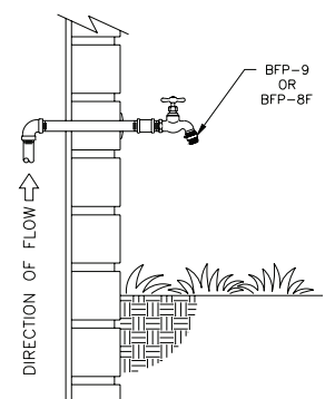
TYPICAL HOSE BIBB INSTALLATION
