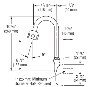
ETF-500-H with Standard Spout and Shower Spray Head
