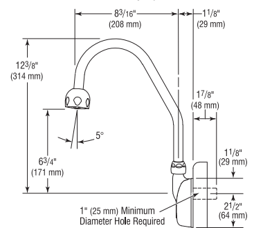
ETF-500-S-H with Surgical Bend Spout and Shower Spray Head
