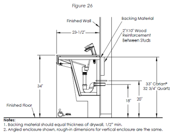
Rough-In (Four Station); Section View
