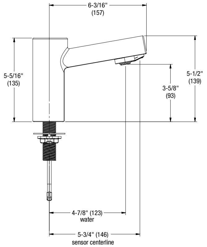
3300 Metro Series
