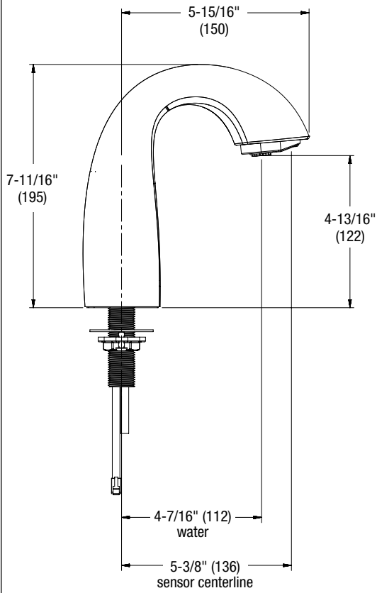
3100 Crest Series
